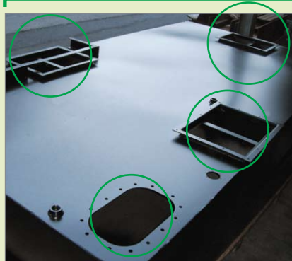
▼ Internal baffles for fuel sloshing control for tanks with capacity > 270 l
