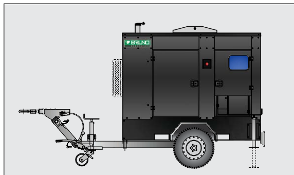
▲ Single-axle road trailer
