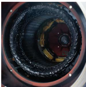
▲ Alternator anti-condensation heater
