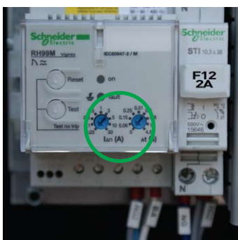
▲ Adjustable ELCB
