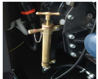
▲ Oil extraction pump
